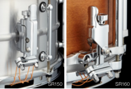
SR160 Snare Strainer Complete SR150 Snare Strainer Complete
