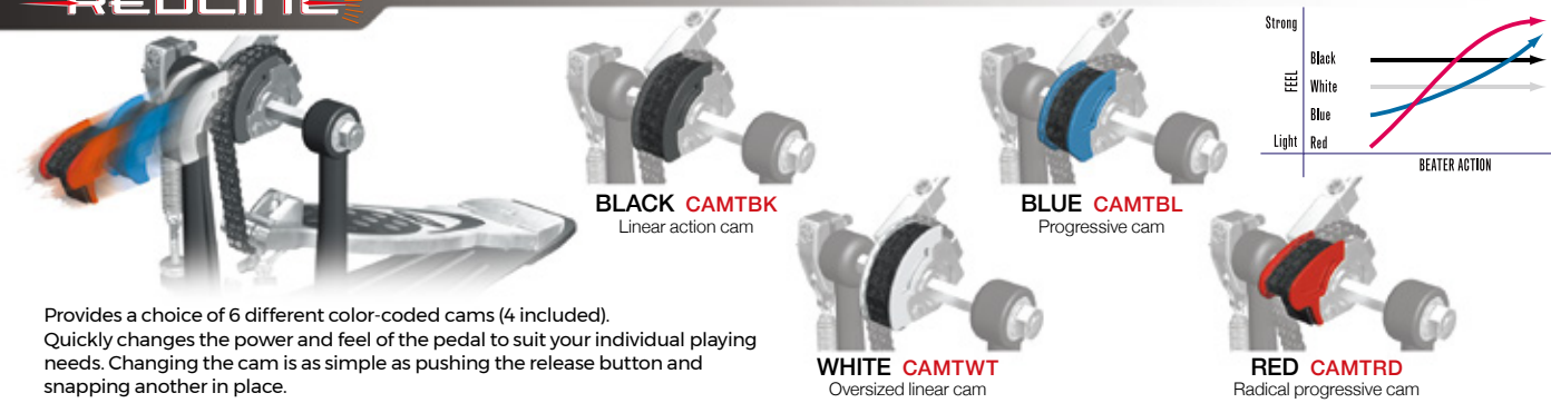
Eliminator: Redline Double Pedal Chain Drive (Shown w/ Included Red Cam Attached) P2052C
